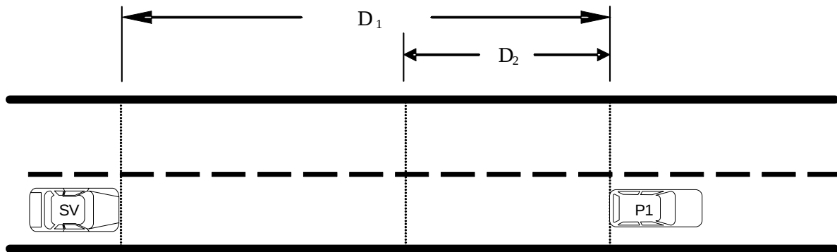
Figure 5: Track Layout for rear-end conflict with a modestly slowing P1 (low P1 deceleration/low time gap) All specific speeds and initial conditions for this test are given in Table 7. Referring to Figure 5, both SV and P1 start in the lane 5 of the skid pad track with an initial gap of D_1 (40 m). Both SV and P1 should reach their respective steady state constant speeds and a constant headway, when the range between SV and P1 is D_2 (30 m).
