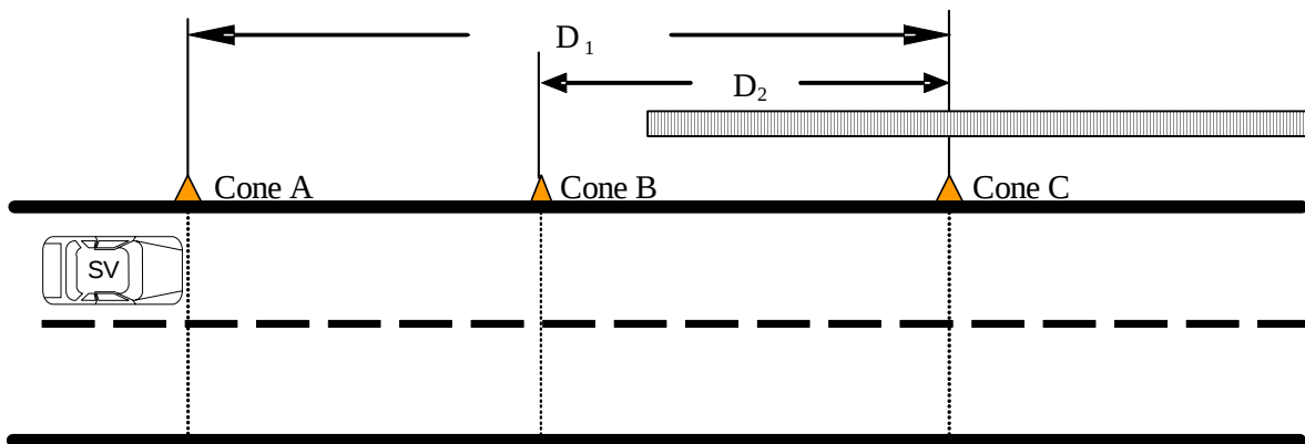
Figure 68: Track Layout for no warning with poor lane keeping.
