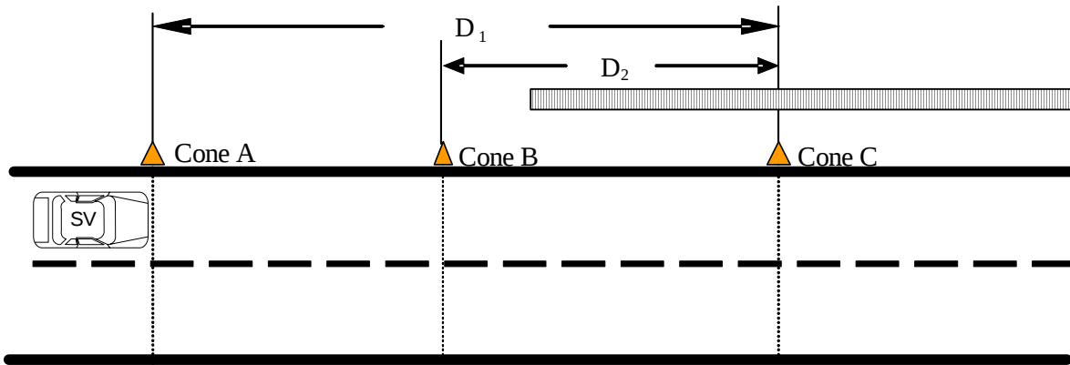
Figure 46: Track Layout for RD toward a barrier with no lane marker.
