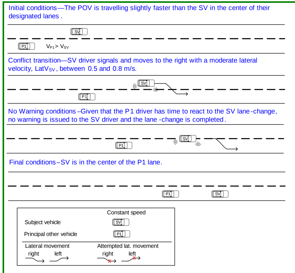
Figure 69: Initial and final conditions for no warning when SV changes lane into adjacent POV that is behind the SV rear bumper.
